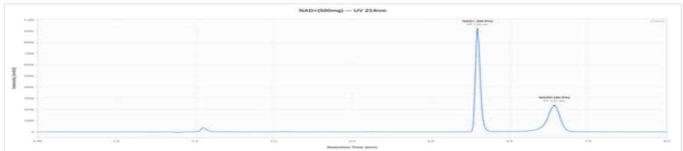
NAD+ 500mg - PS07-NAD500: UV Chromatogram
