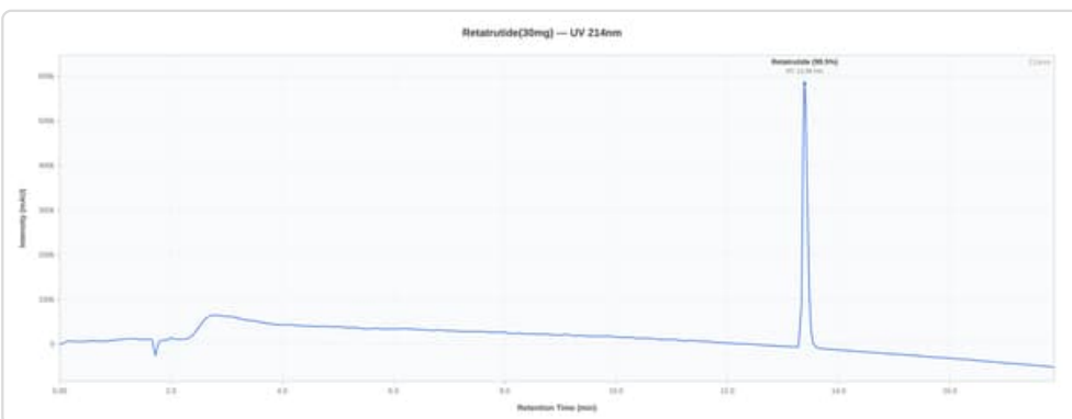
HPLC Chromatogram
